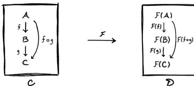
FIGURE 3. A schematic to convey how a covariant functor F from one category \mathcal{C} to another \mathcal{D} acts on its objects and the morphisms between them.
